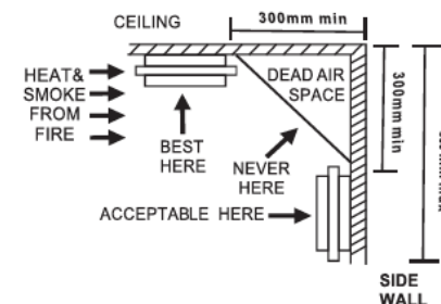
FIGURE 3 – POSITION THE SMOKE ALARM
